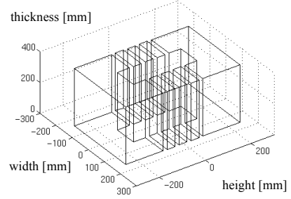
Fig. 11. Optimal inductor design using quality function (2) with a weight of 472 kg.
