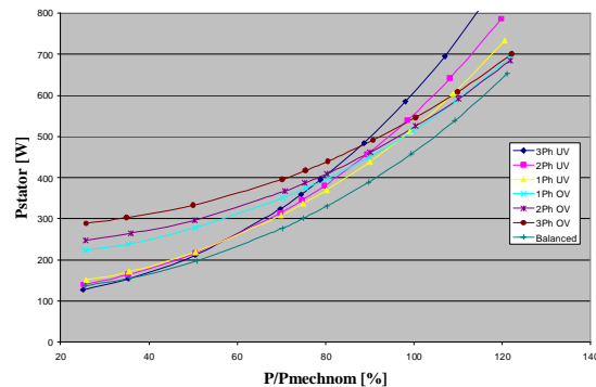
Figure 4: Stator losses for several cases with 4% voltage unbalance EFF3-machine: motor mode
