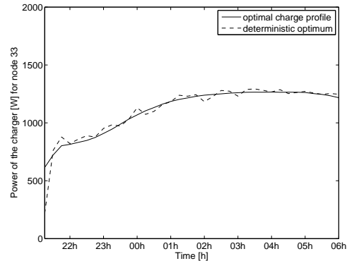
Figure 7: The deterministic optimum and optimal charge profile for node 33.
