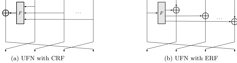
Fig. 1: One round UFN with CRF and ERF
