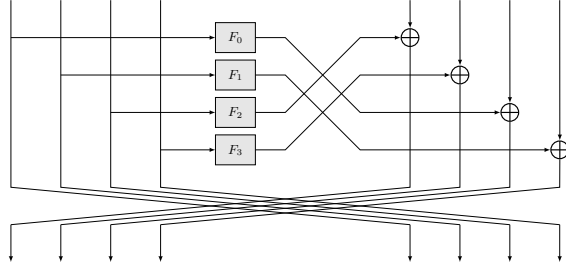
Fig. 2: One round \mathcal{R}_s of an 8-branch Multi-Rotating Feistel network with a rotation by s = 2 .
